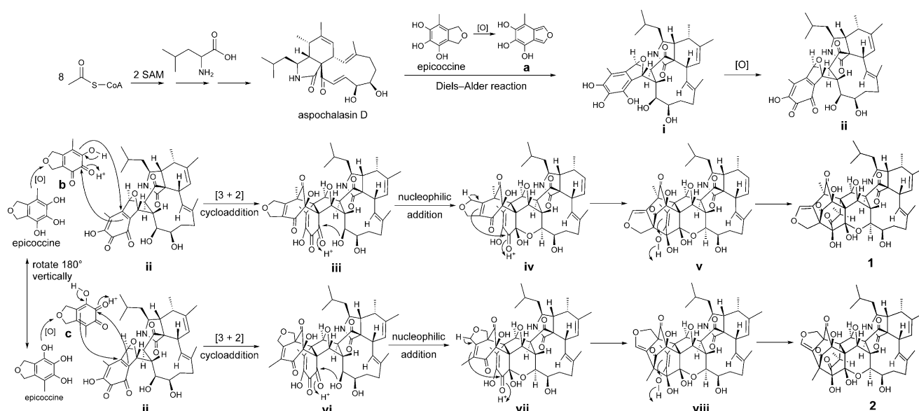
Scheme 2. Plausible biosynthetic pathways of epicochalasin A ( 1 ) and B ( 2 ). CoA = coenzyme A, SAM = S-adenosyl-L-methionine.
